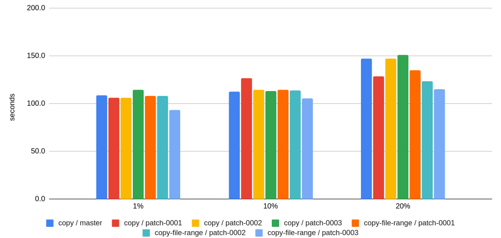
timing / btrfs / with manifest
