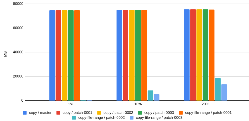
occupied space / xfs / without manifest
