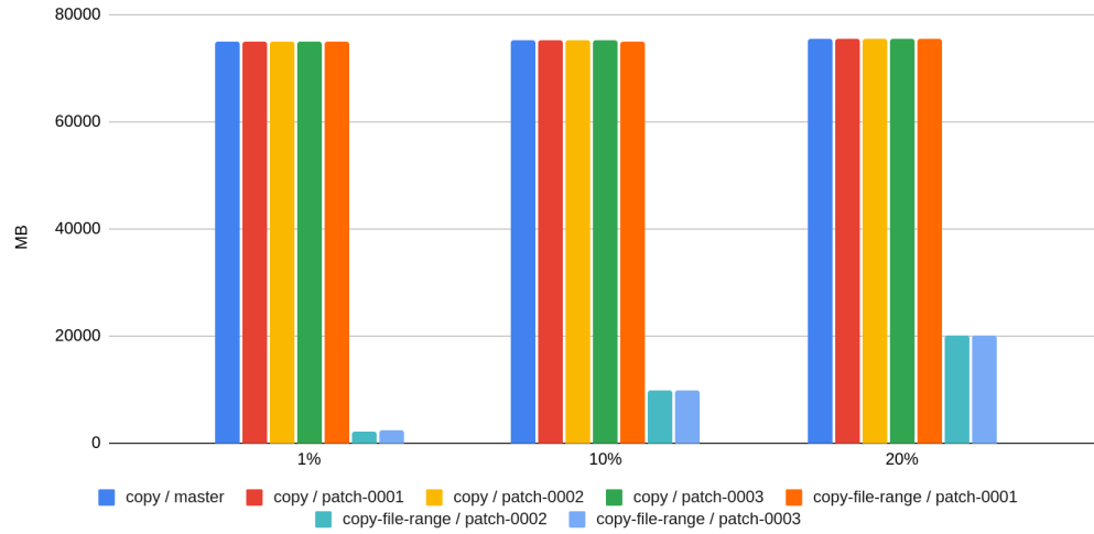
occupied space / btrfs / without manifest
